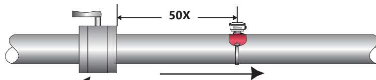
Partially Open Butterfly Valve
